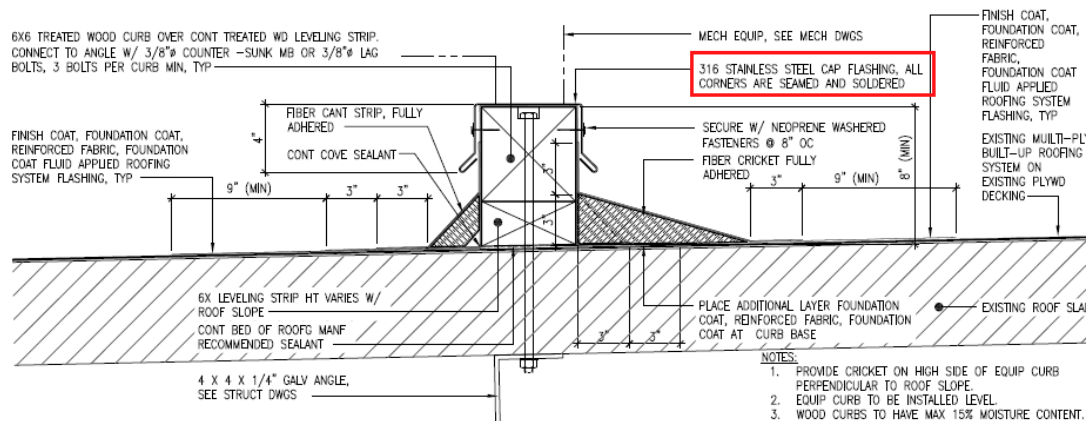
2 EQUIPMENT CURD & FLASHING DETAIL A-3 SCALE: 3" = 1'-0"
